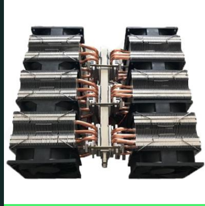
Semiconductor Thermostatic Refrigerator
